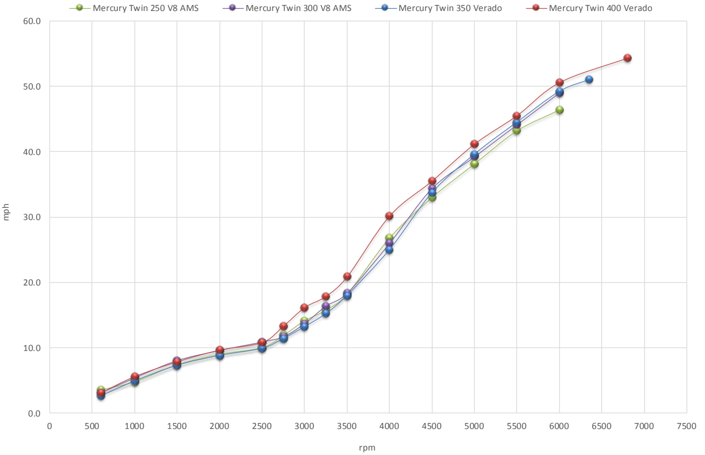
320 Vantage Engine Comparison Graph
